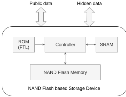
Fig. 2. The organization of a NAND flash storage device with an FTL supporting PD.
