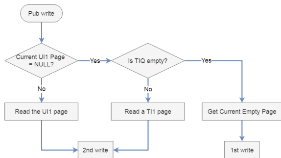
Fig. 7. The diagram about how PEARL allocates physical pages upon accepting a public write request. The priorities of physical pages are: 1st invalid pages in UIQ, 1st invalid page in TIQ, empty pages.
