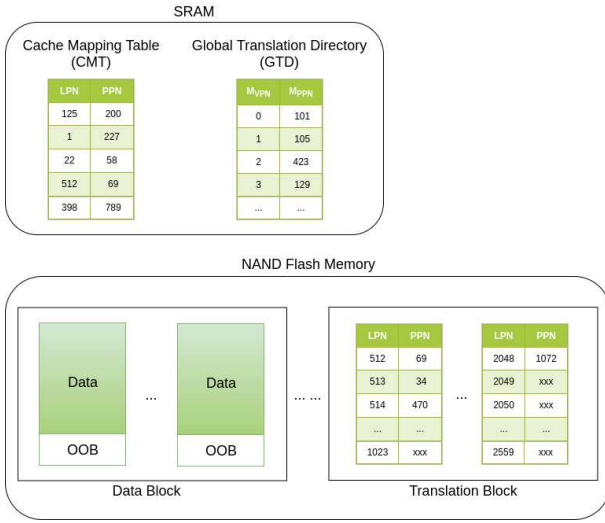
Fig. 1. The organization of DFTL. LPN is the Logical data Page Number, PPN is the Physical Page Number, M_{VPN} is the Virtual Translation Page Number, M_{PPN} is the Physical Translation Page Number.
