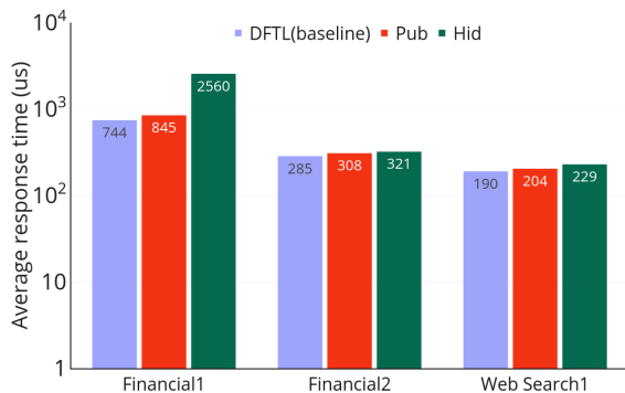
Fig. 9. The average response time for three real-world traces with different FTLs (log scale for the y axis, lower is better).
