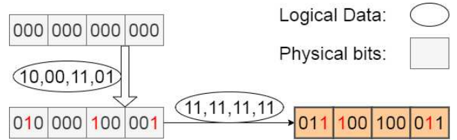
(a) A WOM code allows multiple writes to the same physical locations by flipping some of the bits from 0 to 1. In this example, an initial write of 8 data bits results in setting 3 bits of "1" among 12 physical bits. Then, later in a second write, a completely different set of 8 bits of data can be written to the same locations by setting another 3 bits to 1. In the end, the 12 physical bits 010, 000, 100, 001 represent data 11, 11, 11, 11
