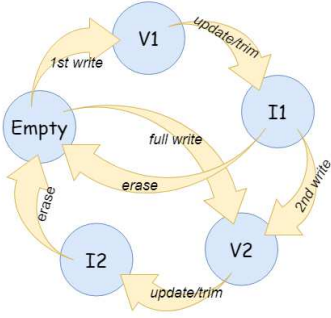
Fig. 6. Page state transition diagram using the 2-write WOM code. A page written twice with public data can transition through all 5 states while a page written once with public and hidden data skips states V1 and I1. It is also possible that a page is recycled right after it is written only once with public data (state I1 to Empty directly).
